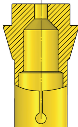
SHORTENED CLAMPING SURFACE
