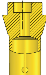
ECCENTRIC, BACK DRILLED CENTER
